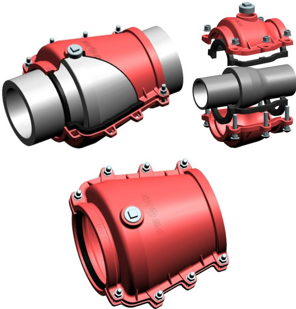
Spigot Socket sealing clamp
